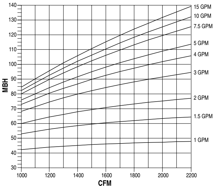
3 Row (multi-circuit)
