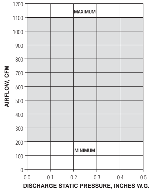
Unit Size 3
