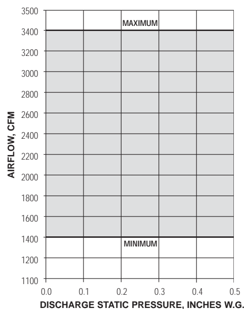
Unit Size 7
