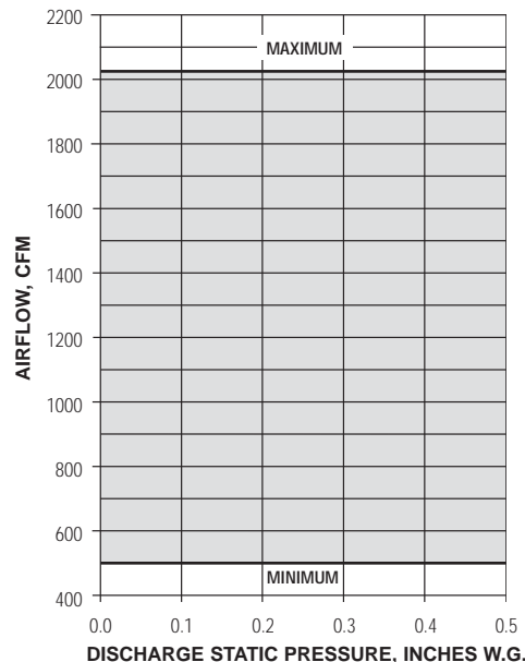
Unit Size 5
