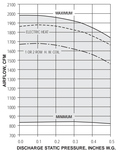
Unit Size 5
