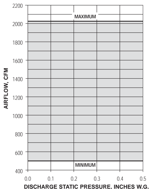
Unit Size 5
