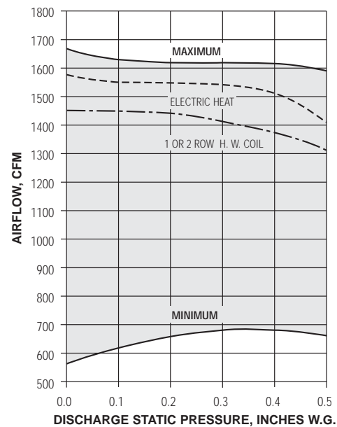
Unit Size 4
