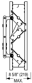
Opposed Blade (Model 1020 Shown)
