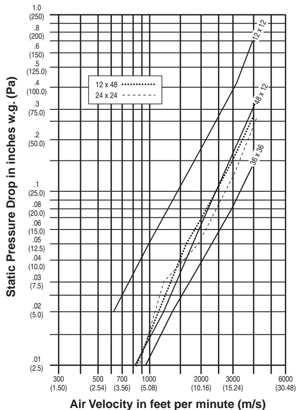
Pressure drop tested per AMCA Standard 500-D-98, Figure 5.3. Data corrected to standard air density of 0.075 lbs/ft 3 .
