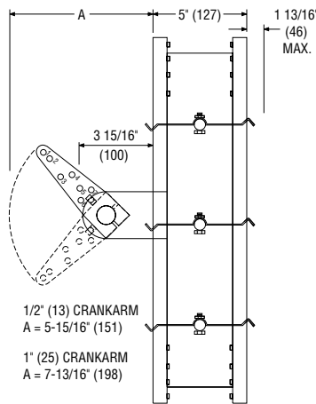
TYPICAL JACKSHAFT
