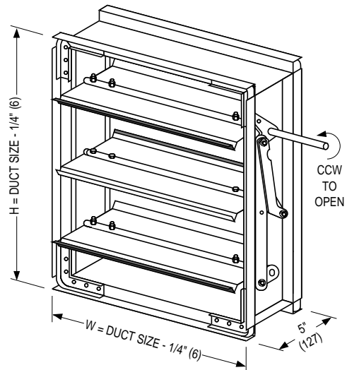
MODEL 1010 WITH 13 GA. FRAME PARALLEL BLADE
