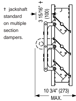
Parallel Blade (Model 1010 Shown)
