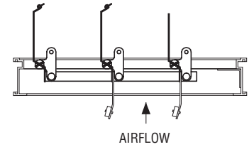
Horizontal Mount – Airflow up (Option HMU) (Available on all frame styles)
