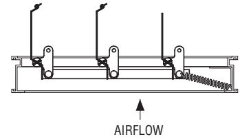
Horizontal Mount – Airflow up only (Option HMU) (Available on all frame styles)
