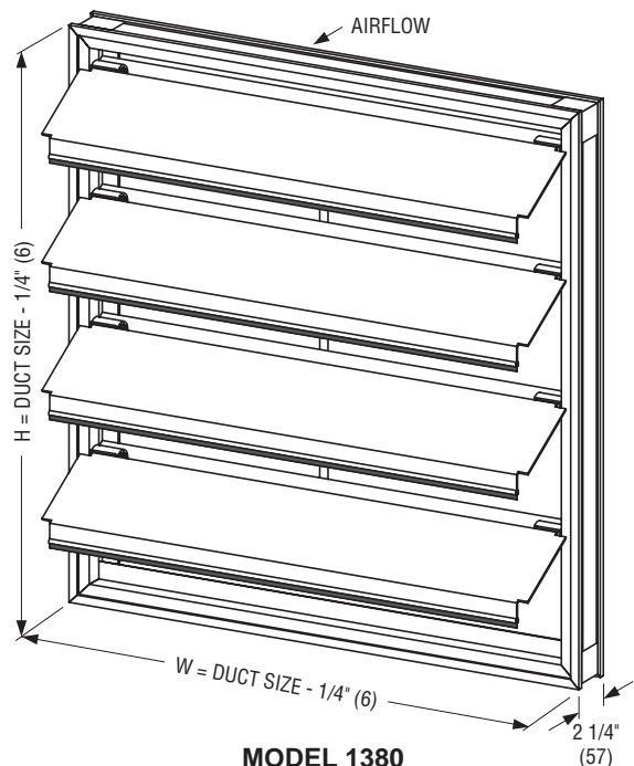
MODEL 1380 (VM Vertical Mount standard)
